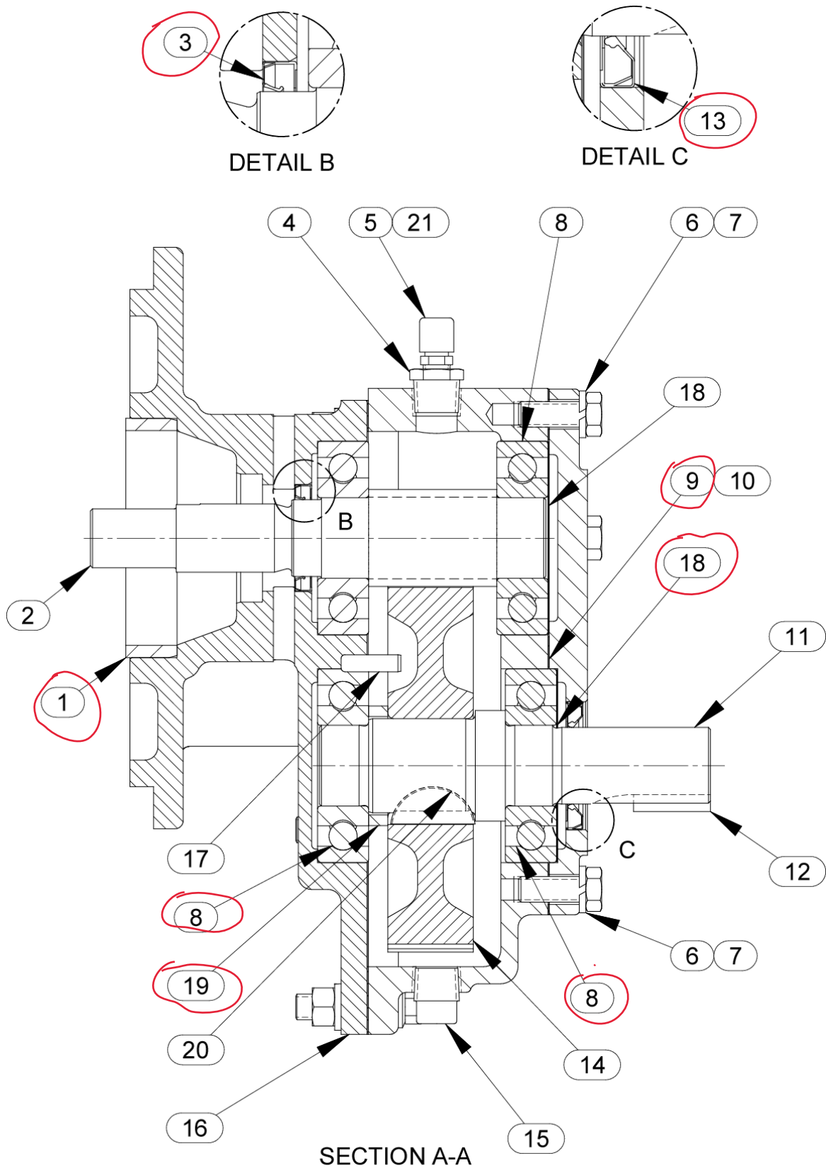
Figure 2. 44161-016 Gearbox Assembly
